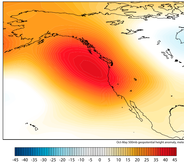
Figure 2. The proximal cause of California's multiyear drought is the remarkable persistence of a region of midtropospheric high pressure known as "The Ridiculously Resilient Ridge." The plotted quantity is the mean cool season 500 mbar geopotential height anomaly (meters) over four consecutive years (i.e., October–May 2012, 2013, 2014, and 2015).
